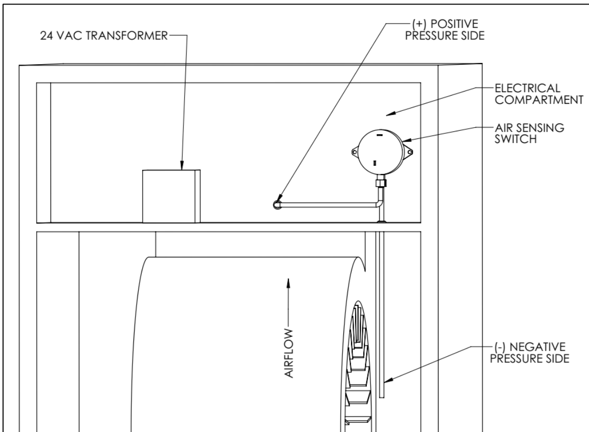
Simplified Typical Installation.
